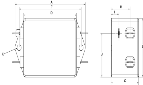
Connection style -3, 1A to 6A types (same dimensions as style -1)
