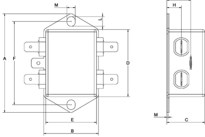
Connection style -1, 8A to 12A types
