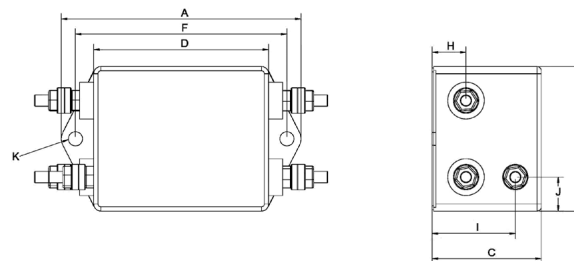
Connection style -6, 16A to 30A types
