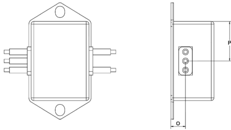
Connection style -6, 16A to 30A types
