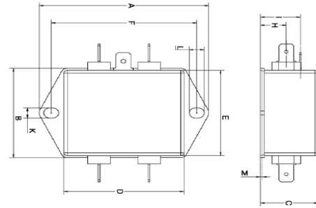
Connection style -1, 3A to 6A types
