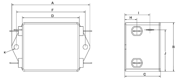
Connection style -3, 8A to 16A types (same dimensions as style-1)
